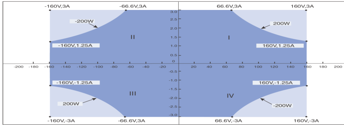
■ Pulse only,maximum pulse on time 1ms,maximum duty cycle 5% ■ Pulse only,maximum pulse on time 400 us,maximum duty cycle 2%
